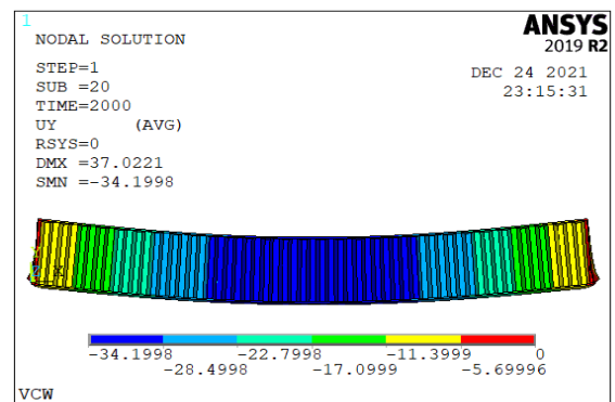
(b) Vertical corrugated web (VCW)
