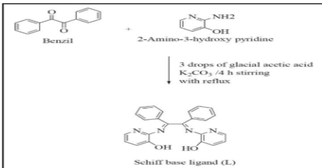
Figure 1 Synthesis of Schiff base ligand
